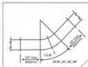
Horizontal Elbows
