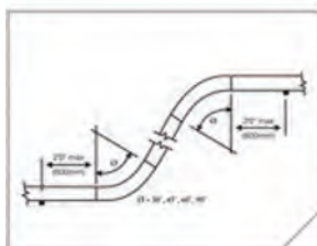
Vertical Elbows
